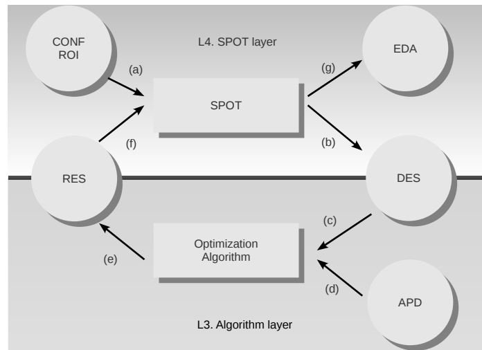
Figure 7: SPOT interfaces. The SPOT loop can be described as follows: Configuration (CONF) and region-of-interest (ROI) files are read by SPOT (a). SPOT generates a design (DES) file (b). The algorithm reads the design file and (c) extra information, e.g., about the problem dimension from the algorithm-problem design (APD) file (d). Output from the optimization algorithm are written to the result (RES) file (e). The result file is used by SPOT to build the prediction model (f). Data can be used by exploratory data analysis (EDA) tools to generate reports, statistics, visualizations, etc. (g)
