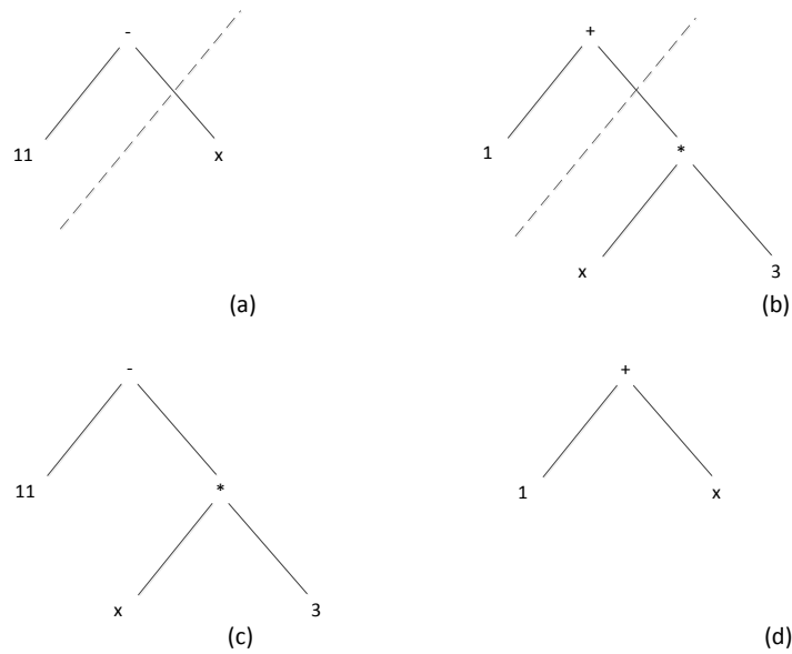
Figure 2: Crossover via sub-tree exchanging applied to two GP individuals (a) and (b), which are represented as binary trees. The first tree represents the S-expression '-(11 x)' , the second tree represents '+(1 (* (x 3)))' . The dashed lines denote the positions, where crossover takes place. Two offspring are created: (c), which represents '-(11 (* (x 3)))' and (d), which represents the S-expression '+(1 x)' .
