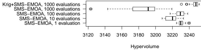
Fig. 10: Boxplots for the optimization experiments with the stochastic simulation. The x-axis shows hypervolume of the estimated fronts, validated by 10,000 runs for each point. Higher values are better. Evaluation numbers refer to the repeated evaluation of each point.
