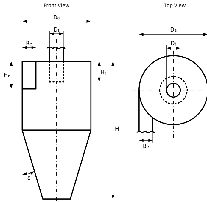
Fig. 1: Schematic representation of a cyclone dust separator.
