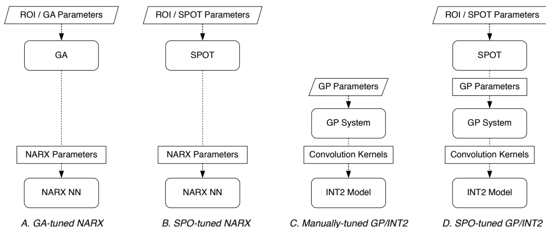
Figure 1: Case study architecture overview. This figure illustrates the setup of the four case studies, see Sec. 3. From left to right: The neuro-evolution approach (A), which is directly compared to the SPO-tuned neural network (B). The setup of the manually-tuned GP/INT2 approach (C), which is directly compared to the SPO-tuned GP/INT2 approach (D).
